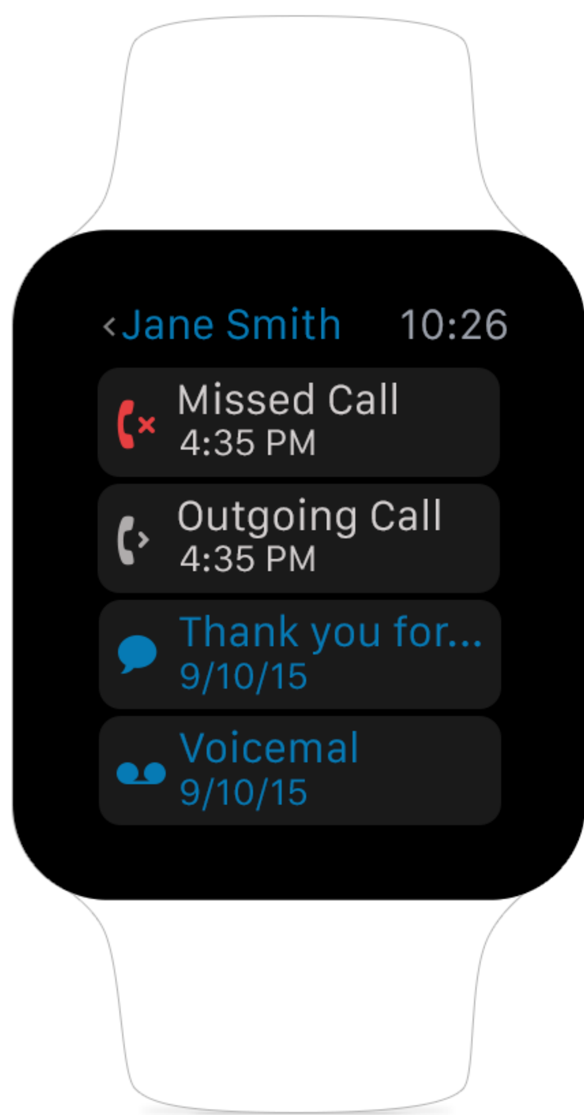
1. Timeline
