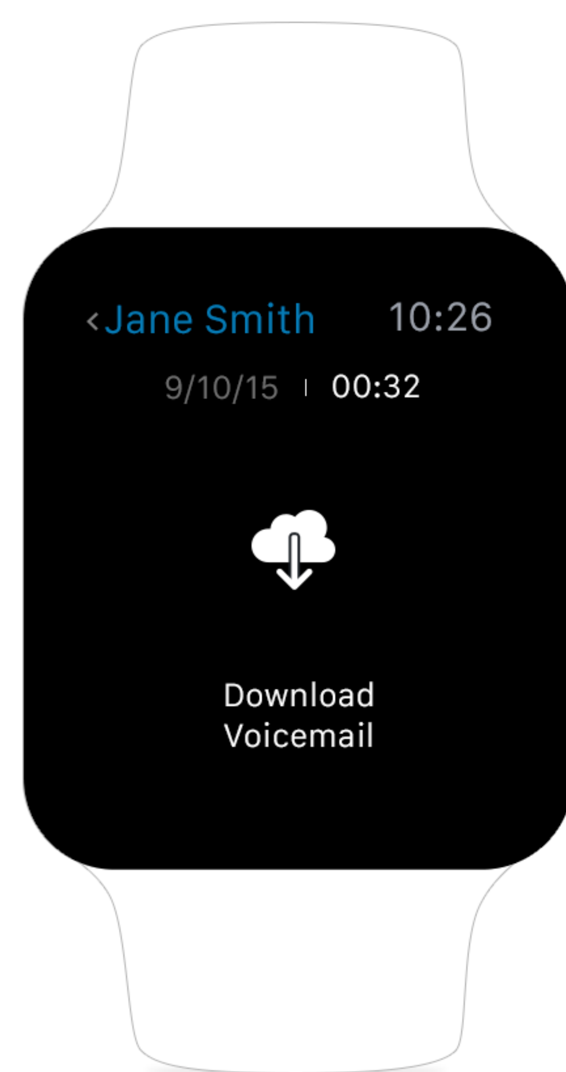
3. Download Voicemail
