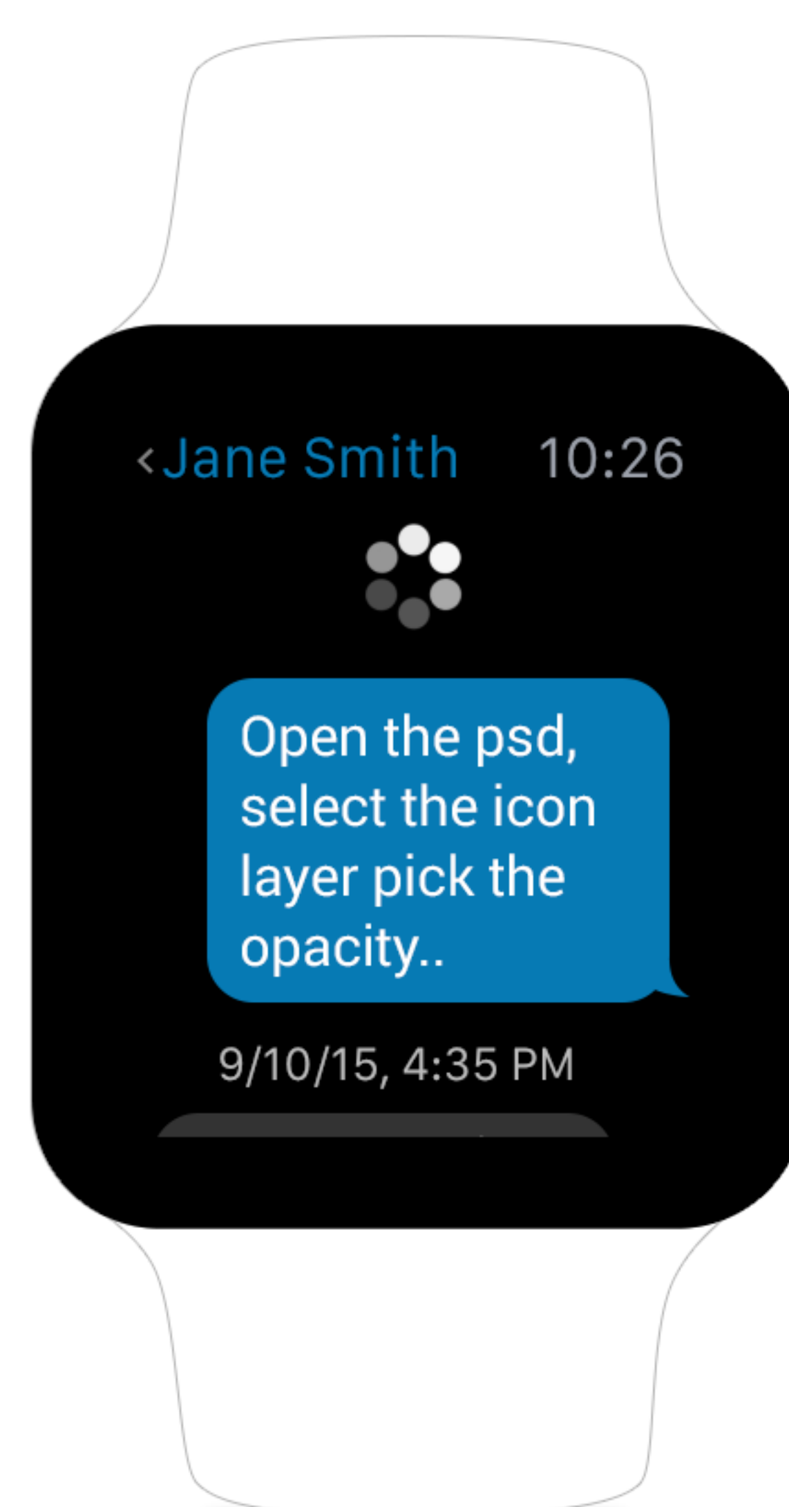
10. Loading
