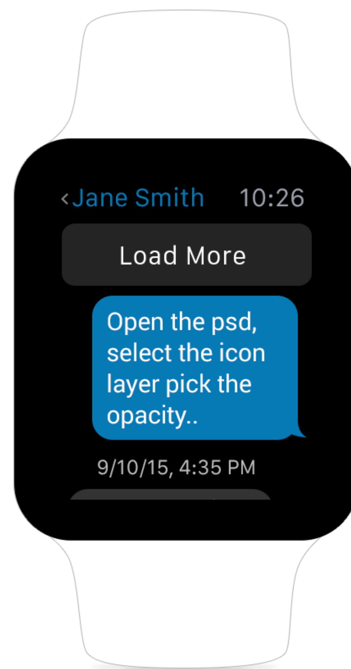
7. Load More
