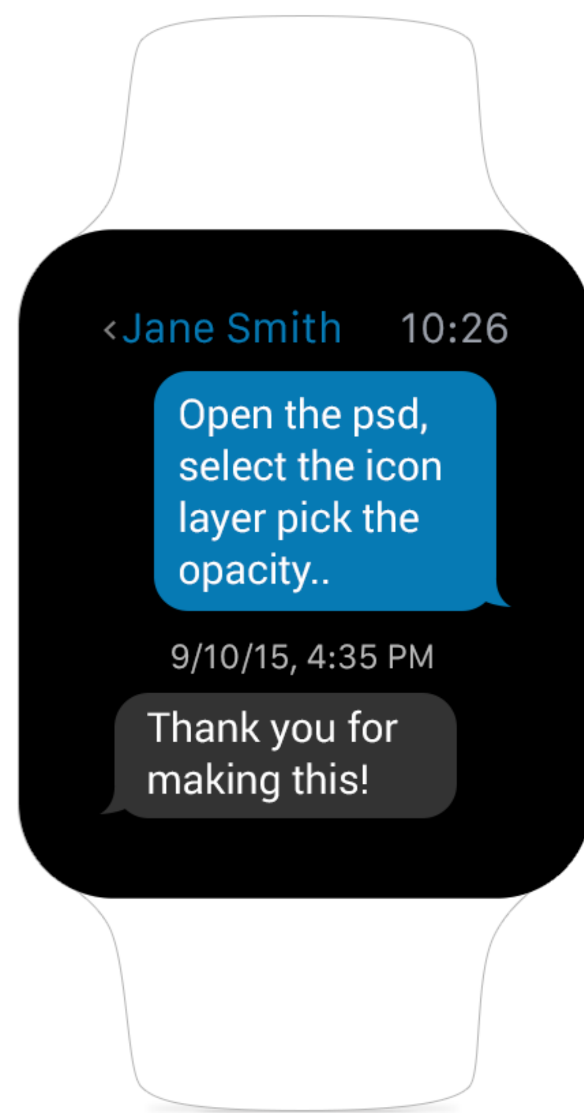
2. Conversation screen
