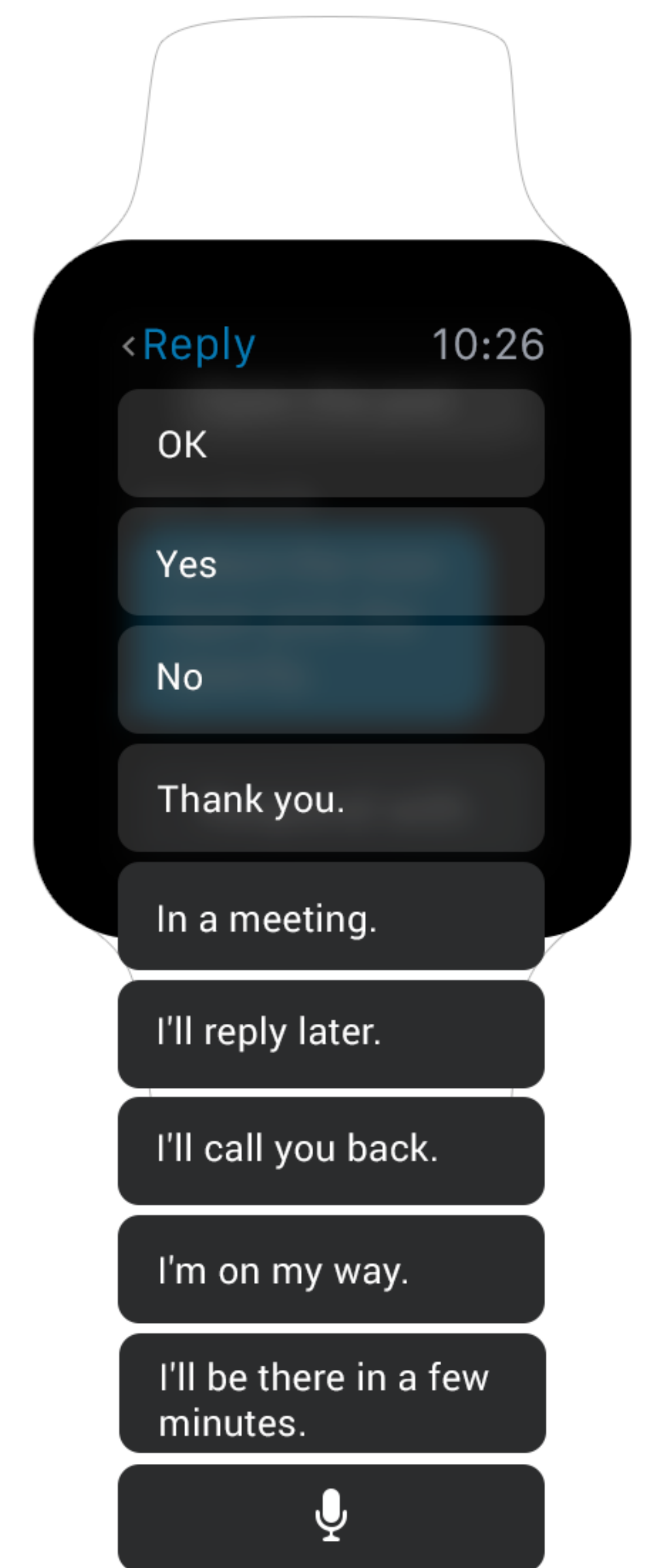
4. Reply
