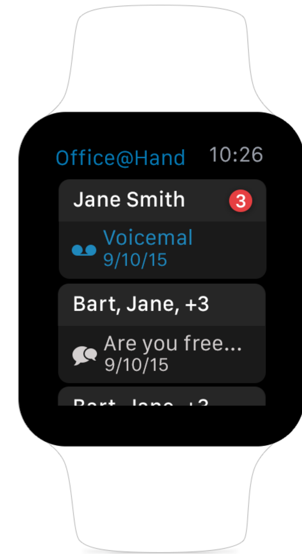
4. View
