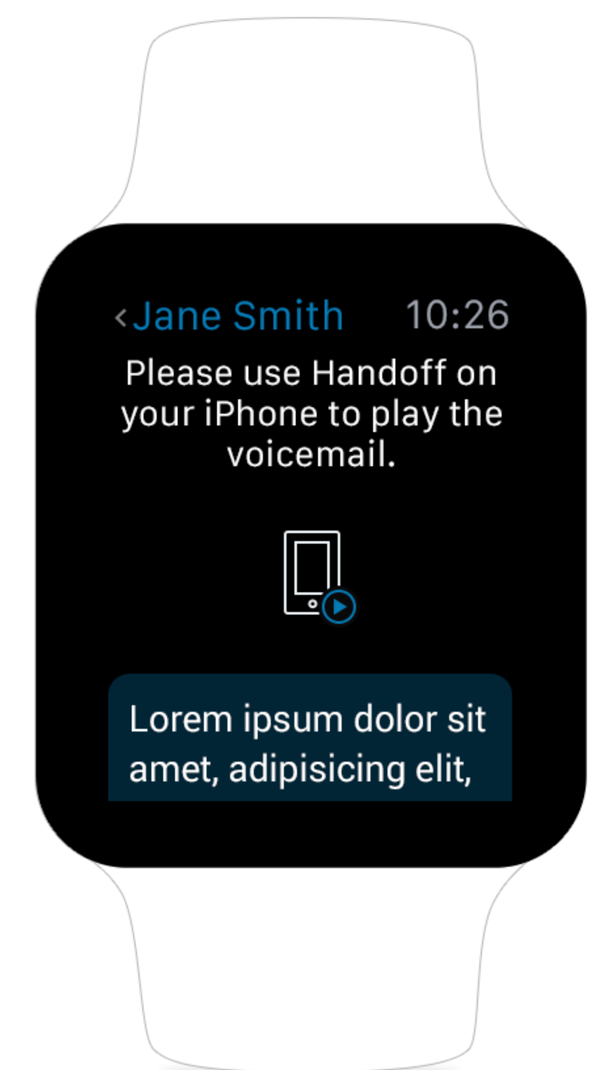
6. Play
