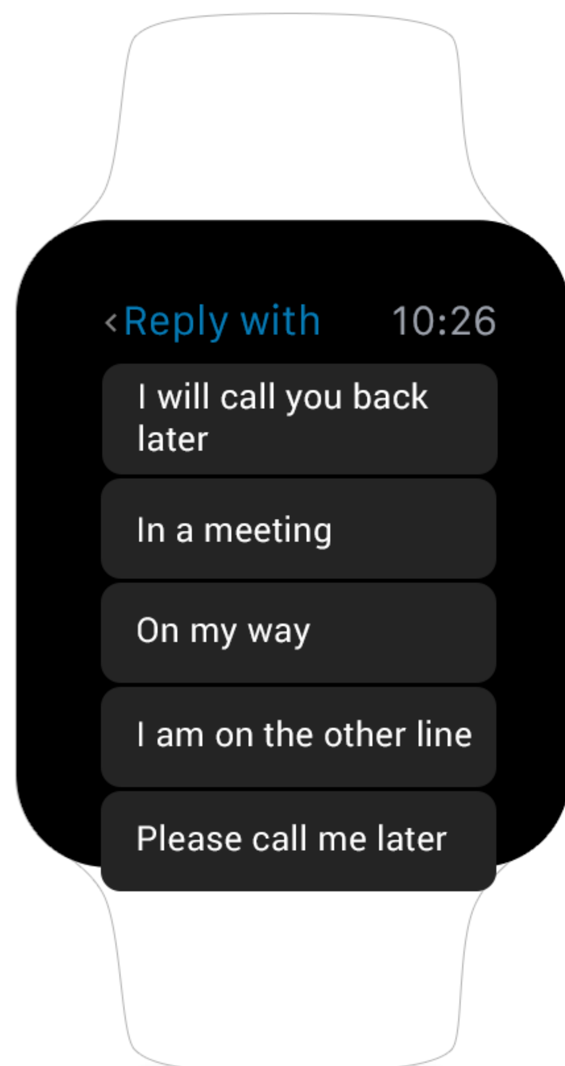
5. Reply with
